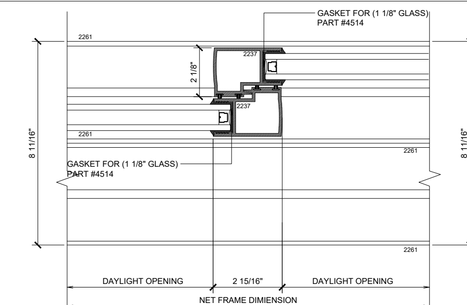
4 VERTICAL MAX SLIDING DOORS (OXXX-XXXO) SCALE: 6"=1'-0"
