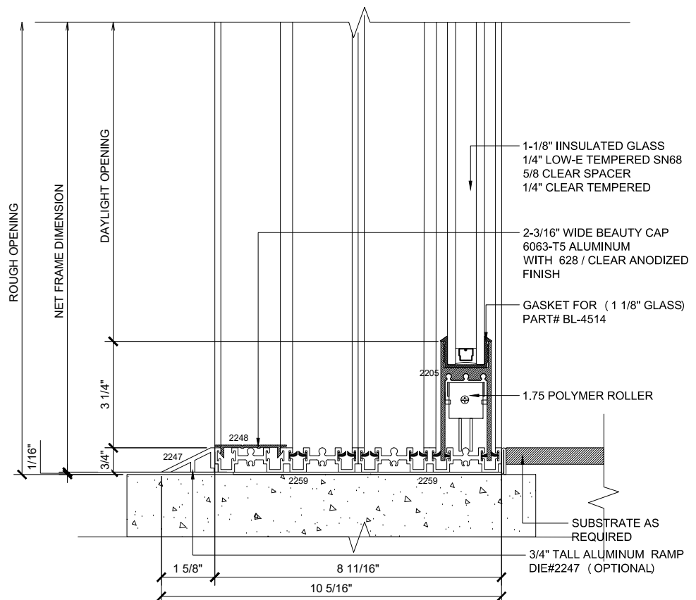
8 SILL (@SLIDER)
