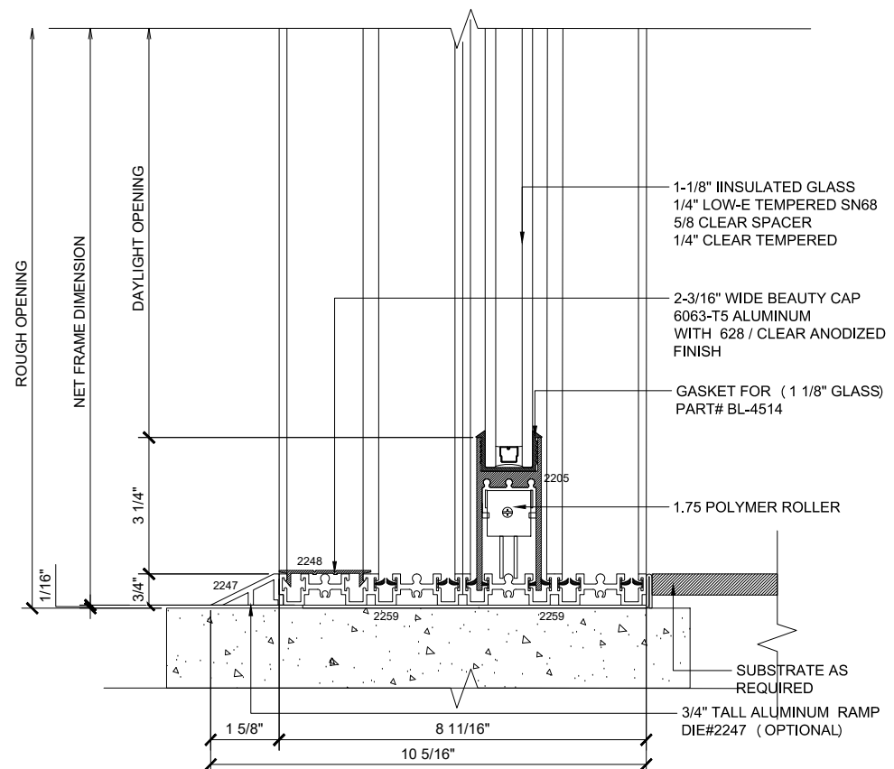
6 SILL (@SLIDER)
