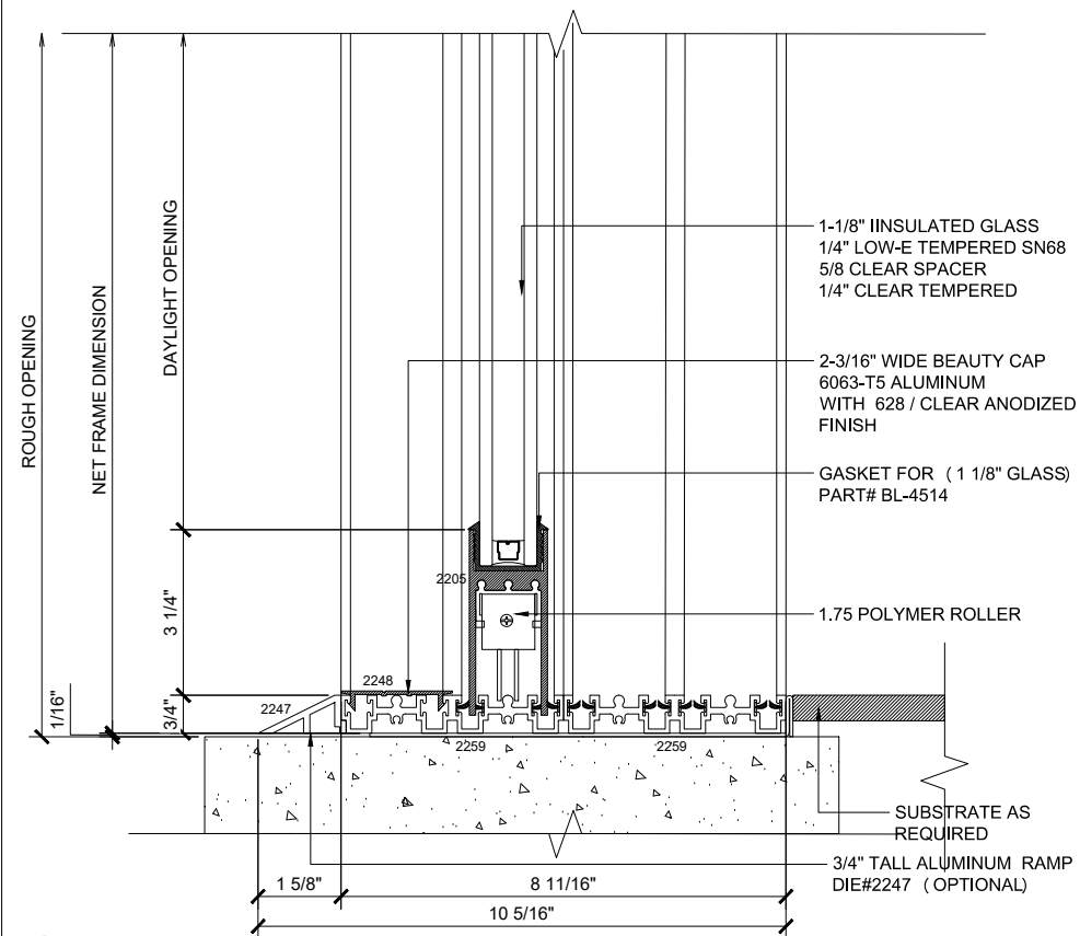
14 SILL (@SLIDER)
