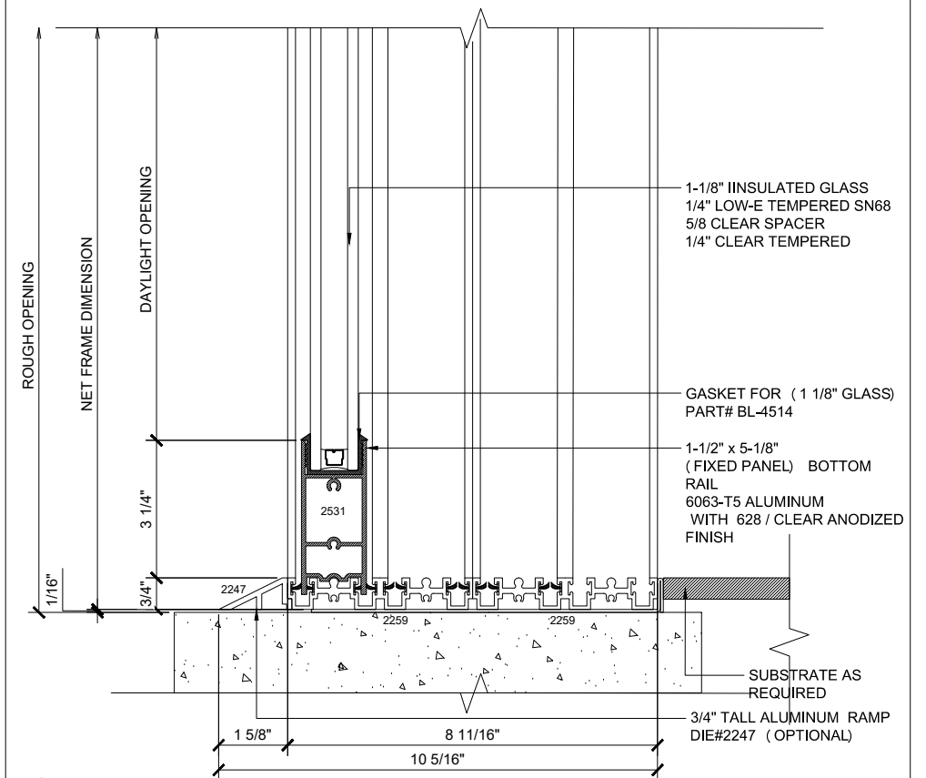
16 SILL (@FIXED)
