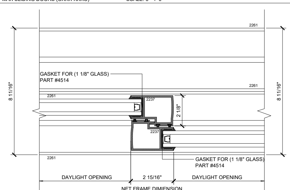
8 VERTICAL MAX SLIDING DOORS (OXXX-XXXO) SCALE: 6"=1'-0"
