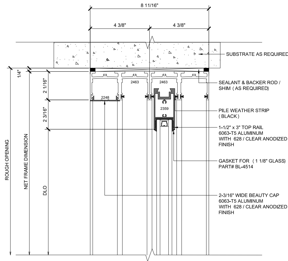
11 HEAD (@SLIDER)
