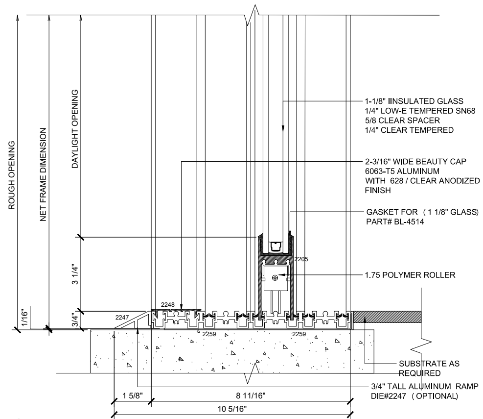
12 SILL (@SLIDER)
