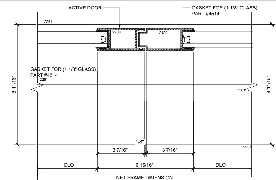
5 VERTICAL MAX SLIDING DOORS (OXXX-XXXO) SCALE: 6"=1'-0"
