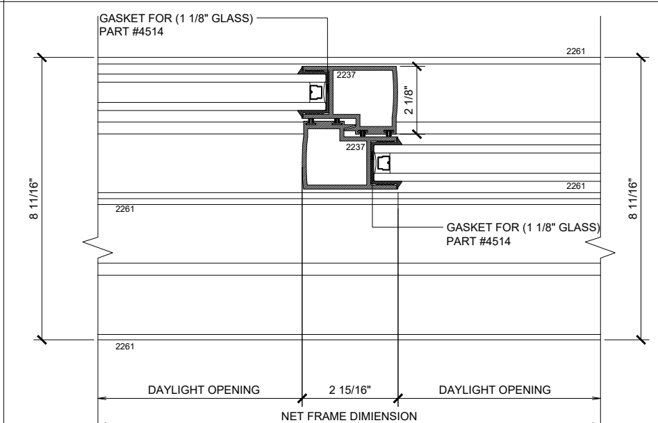
6 VERTICAL MAX SLIDING DOORS (OXXX-XXXO) SCALE: 6"=1'-0"
