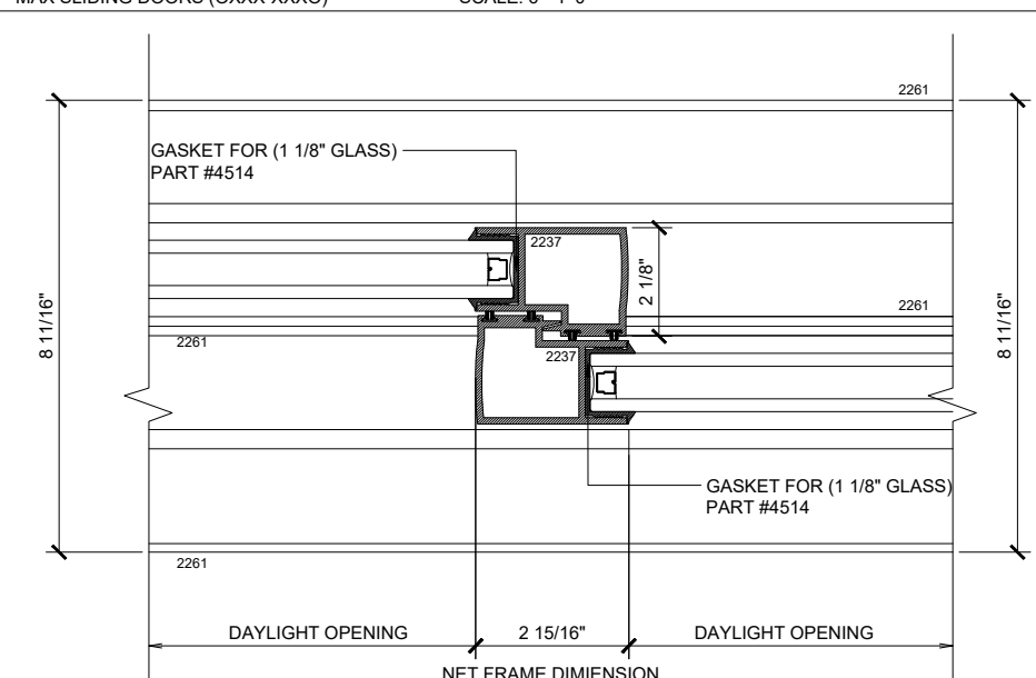
7 VERTICAL MAX SLIDING DOORS (OXXX-XXXO) SCALE: 6"=1'-0"
