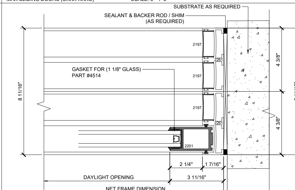
9 JAMB MAX SLIDING DOORS (OXXX-XXXO) SCALE: 6"=1'-0"
