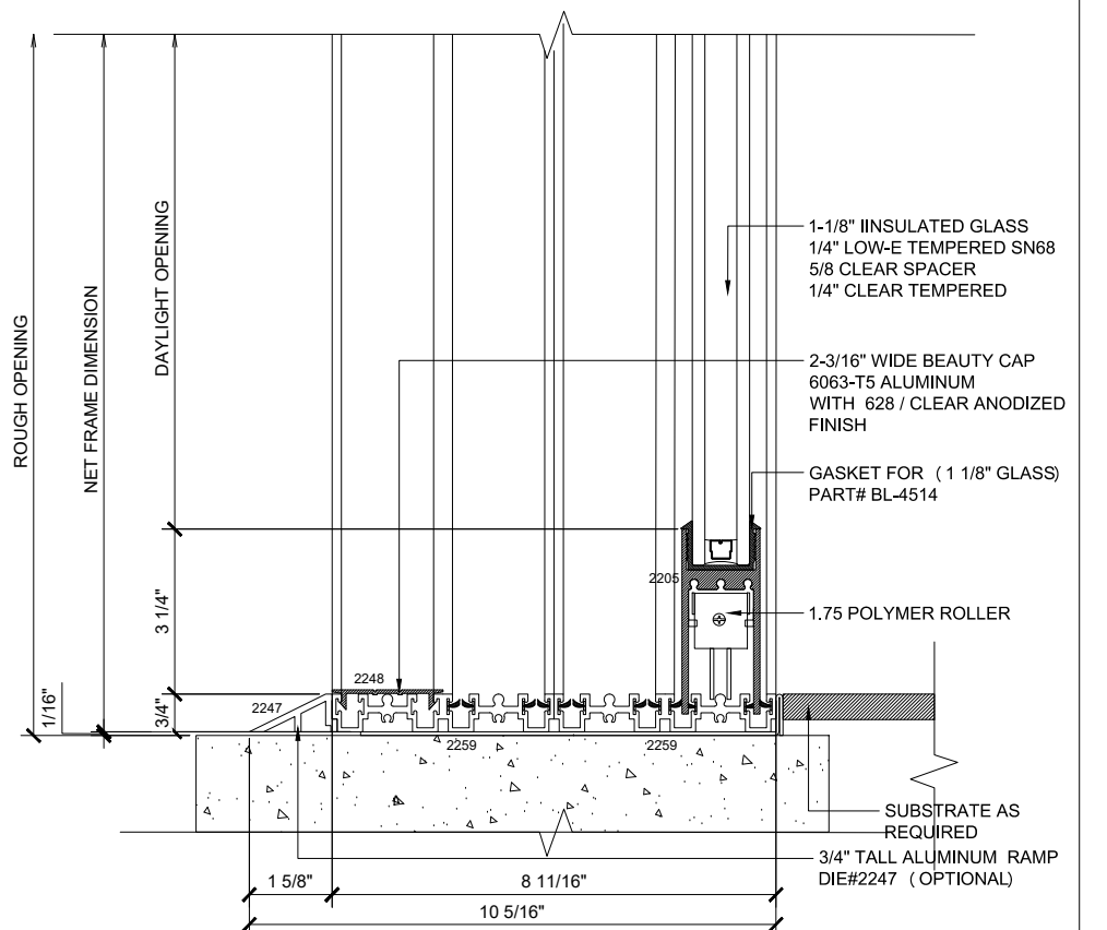
10 SILL (@SLIDER)
