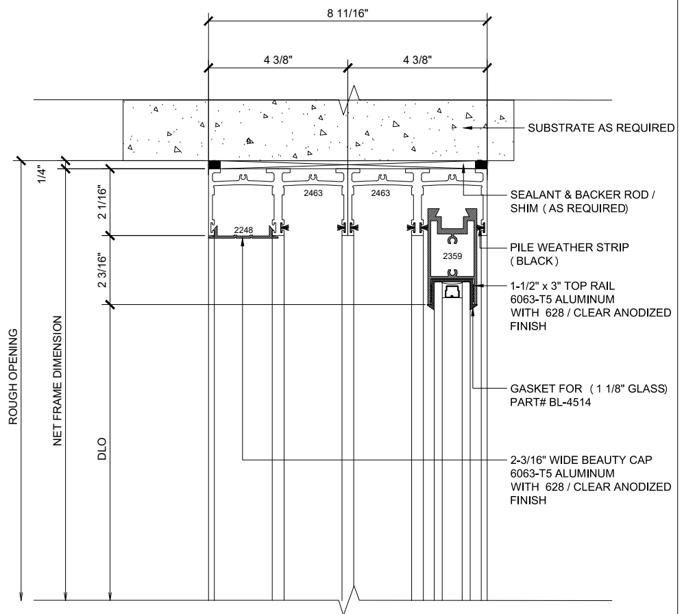
9 HEAD (@SLIDER)
