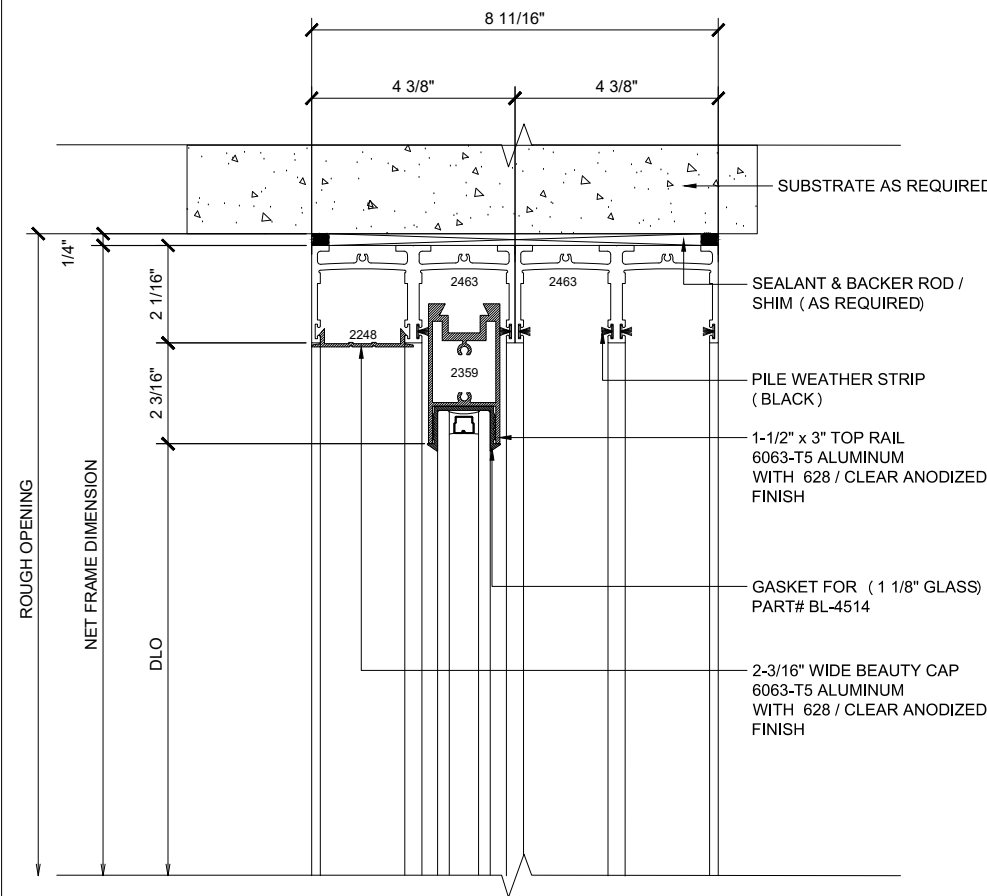
13 HEAD (@SLIDER)
