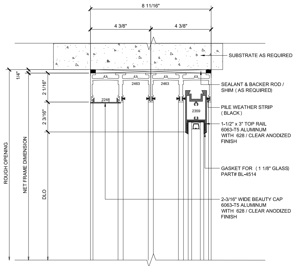
7 HEAD (@SLIDER)
