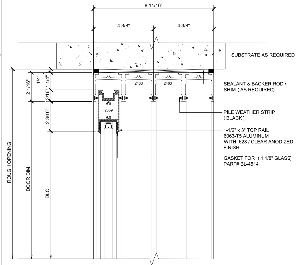
15 HEAD (@FIXED)
